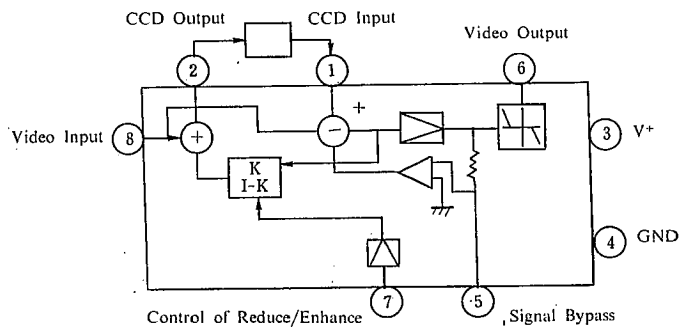
Fig. 2 Block Diagram
