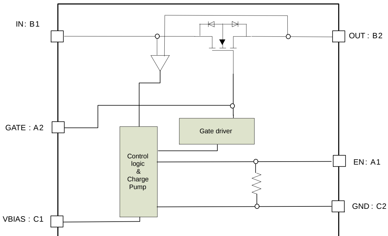
Figure 3. NCP456R Block Diagram – NCP456R Version
