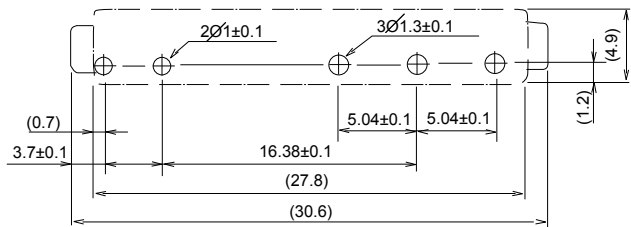
PC Board Mounting Hole Layout (BOTTOM VIEW)
