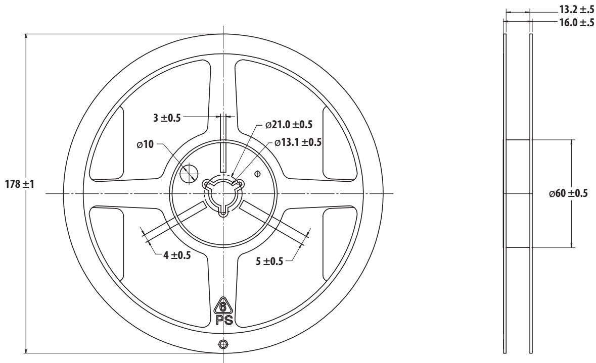
Figure 31 Reel Dimensions
