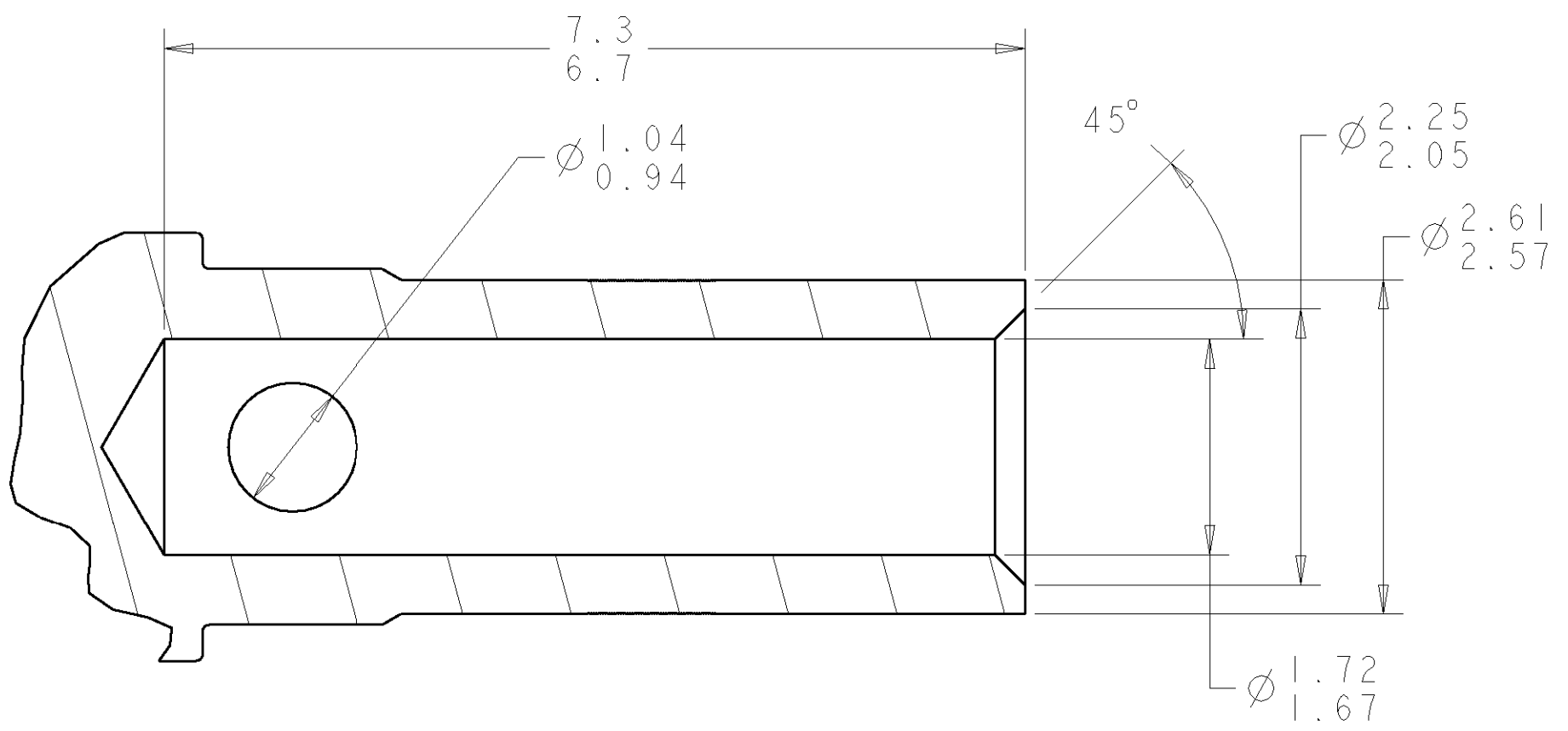
SECTION K-K
