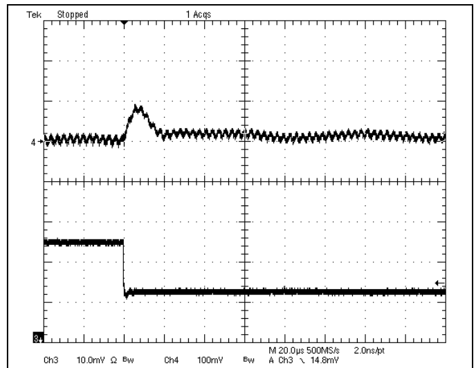
Fig-3.3V-7: Output voltage response for V_{out}=3.3V to negative load current step change from 5A to 2.5A with slew rate of -5A/us at V_{in}=12V . C_o=47\mu F \times 2 ceramic. Top trace: output voltage (100mV/div.) Bottom trace: load current (2A/div.) Time scale: 20us/div.
