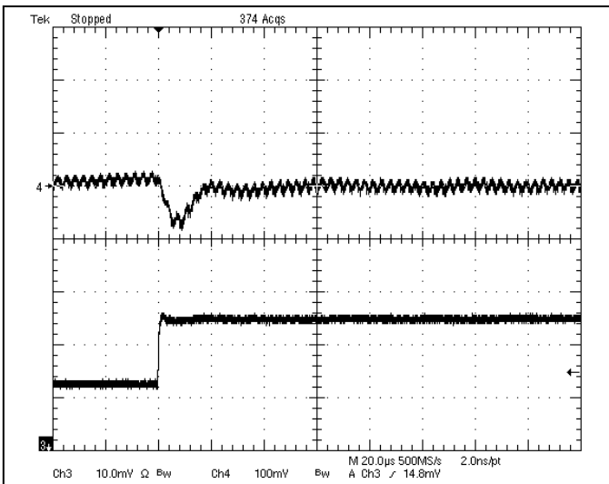
Fig-3.3V-6: Output voltage response for V_{out}=3.3V to positive load current step change from 2.5A to 5A with slew rate of 5A/us at V_{in}=12V . C_o=47\mu F \times 2 ceramic. Top trace: output voltage (100mV/div.) Bottom trace: load current (2A/div.) Time scale: 20us/div.
