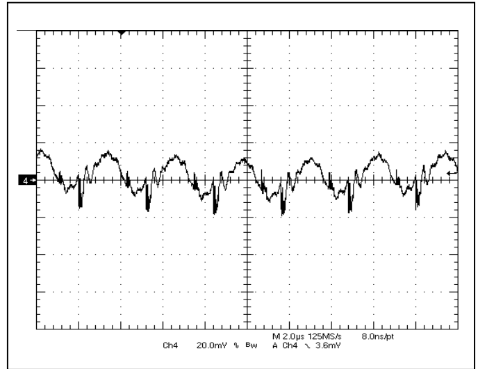
Fig-3.3V-5: Output voltage ripple (20mV/div.) for V_{out}=3.3V at full rated load current into a resistive load with external capacitance 47\mu F \times 2 ceramic + 1uF ceramic at V_{in}=12V . Time scale: 2 us/div.
