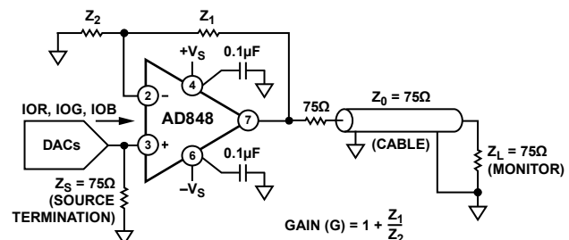
Figure 9. AD848 As an Output Buffer
