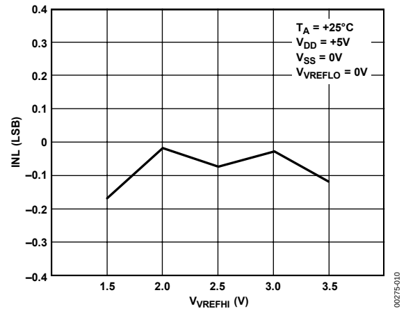
Figure 9. INL vs. V_{REFHI} (+5 V)
