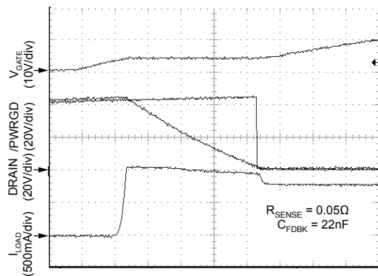
Turn-On Response
