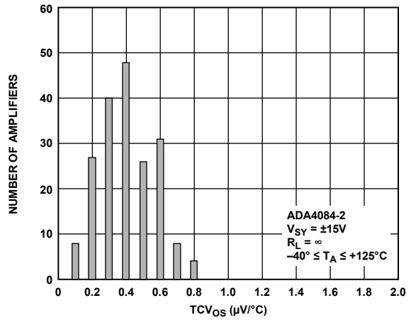
Figure 56. TCV 0s Distribution, SOIC and MSOP
