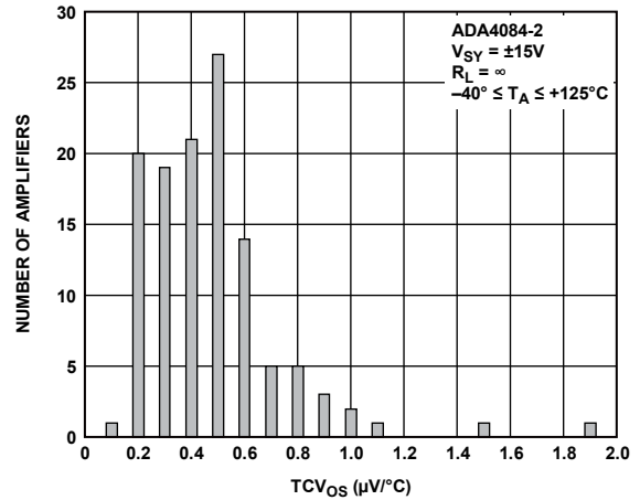
Figure 57. TCV 0s Distribution, LFCSP
