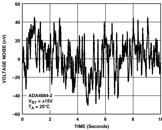
Figure 73. Voltage Noise 0.1 Hz to 10 Hz
