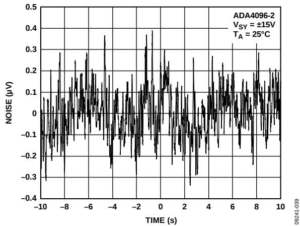
Figure 44. Input Voltage Noise, 0.1 Hz to 10 Hz Bandwidth
