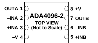
Figure 1. 8-Lead, MSOP (RM-8), ADA4096-2
