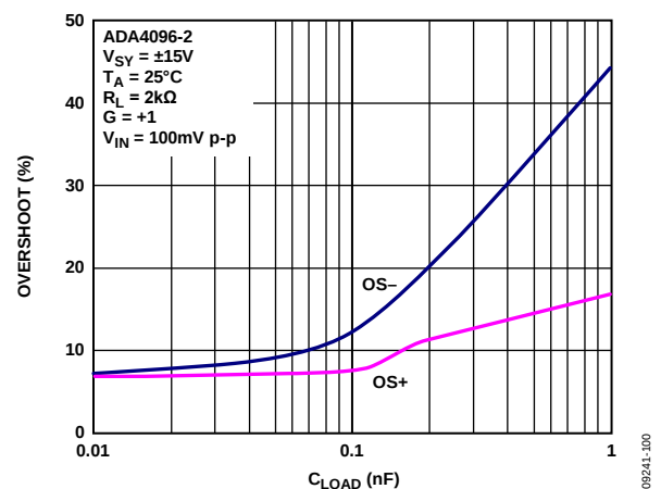
Figure 49. Overshoot vs. Load Capacitance
