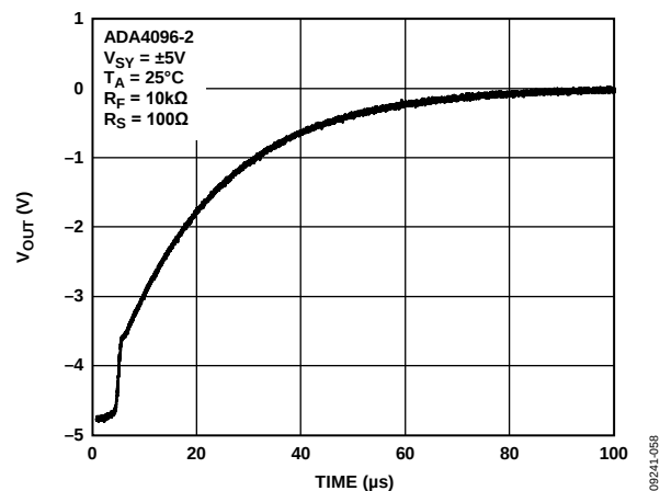
Figure 31. Negative Overload Recovery
