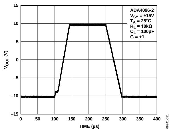
Figure 40. Large Signal Transient Response
