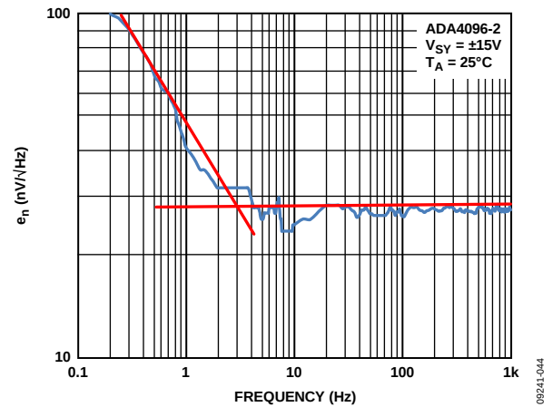
Figure 48. Voltage Noise Density
