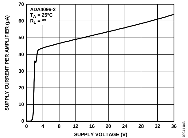
Figure 47. Supply Current vs. Supply Voltage
