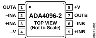
Figure 4. 8-Lead, MSOP (RM-8), ADA4096-2
