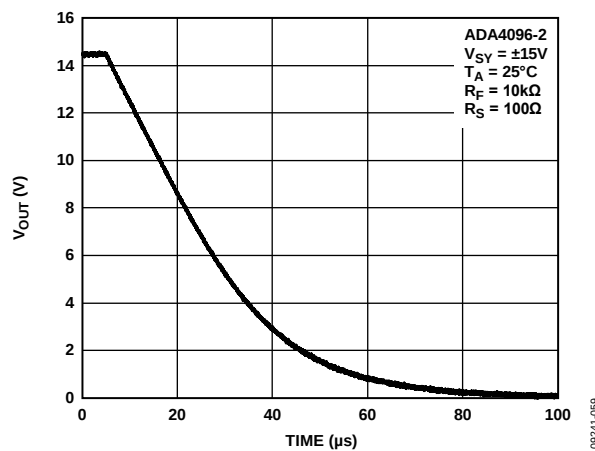
Figure 42. Positive Overload Recovery
