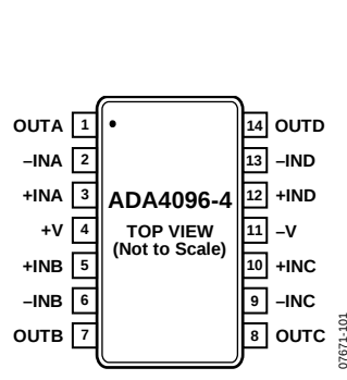
Figure 6. 14-Lead TSSOP (RU-14), ADA4096-4
