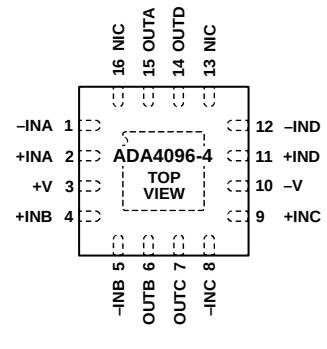
Figure 7. 16-Lead LFCSP (CP-16-27), ADA4096-4
