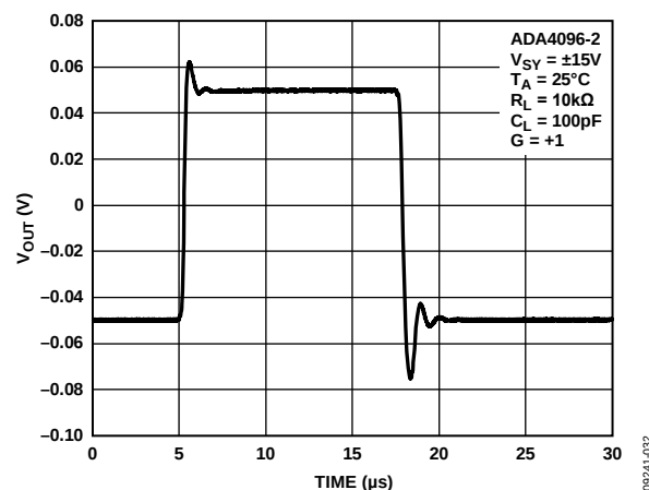
Figure 41. Small Signal Transient Response
