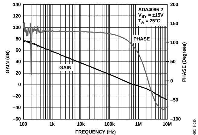
Figure 36. Open-Loop Gain and Phase vs. Frequency
