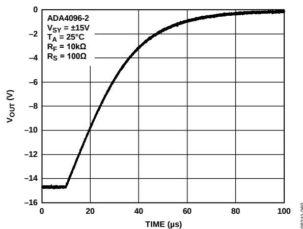
Figure 43. Negative Overload Recovery
