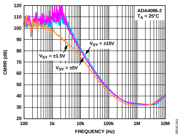
Figure 46. CMRR vs. Frequency
