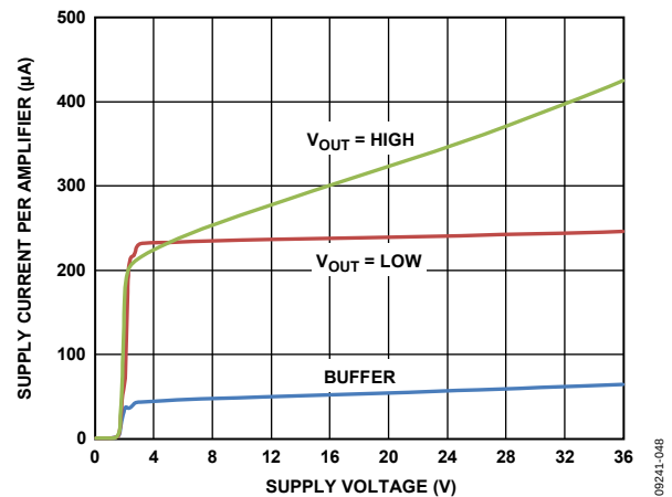
Figure 53. Comparator Supply Current
