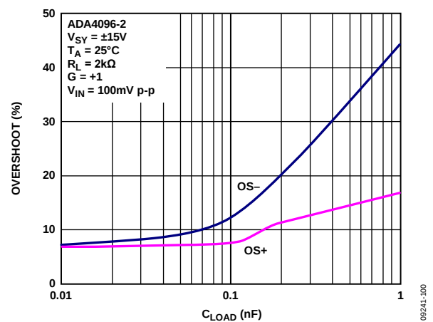
Figure 49. Overshoot vs. Load Capacitance
