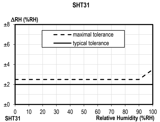
Figure 3 Tolerance of RH at 25°C for SHT31
