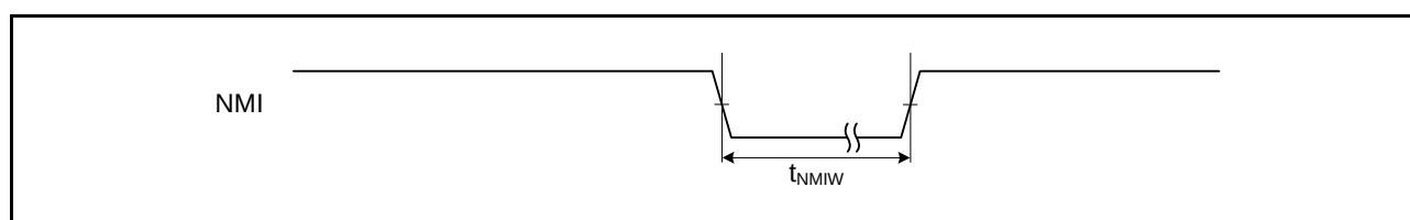
Figure 5.6 NMI Interrupt Input Timing
