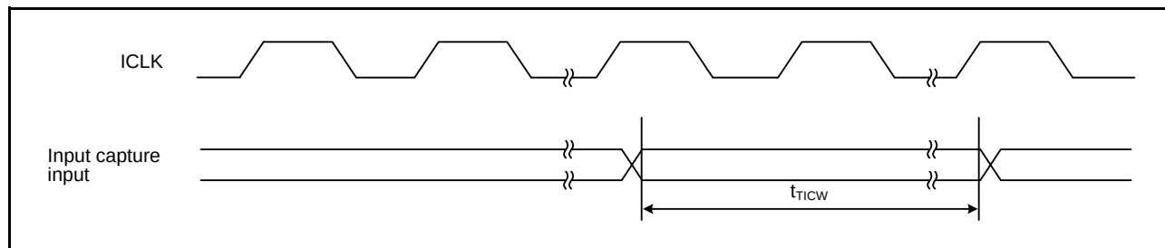
Figure 5.16 MTU3 Input/Output Timing
