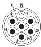
Schematic diagram
