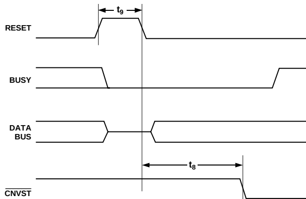
Figure 36. RESET Timing
