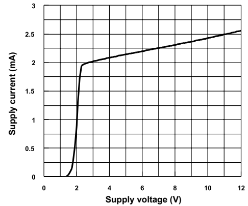
Figure 4. Total supply current vs. supply voltage
