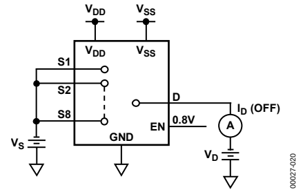
Figure 20. I_D (OFF)
