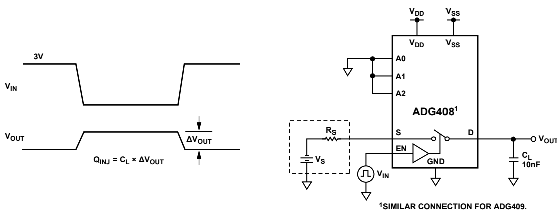
Figure 25. Charge Injection
