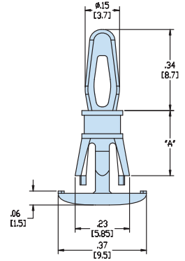
BAYONET SNAP FIT 8,7 / REVERSE BUTTON LOCK
