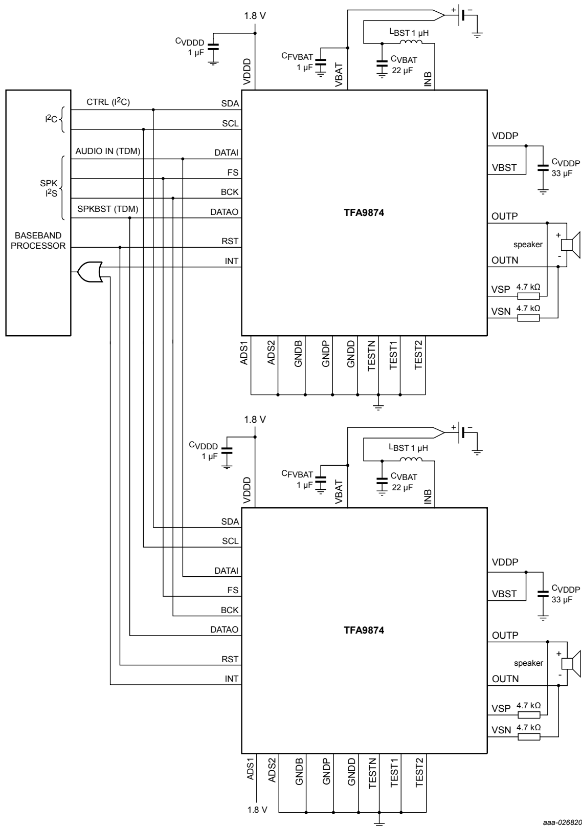
Figure 7. Typical stereo application
