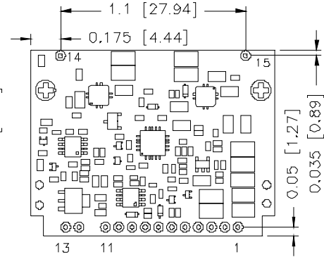
BOTTOM VIEW UNIT:INCH [MM]
