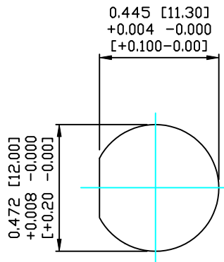
PANEL CUTOUT
