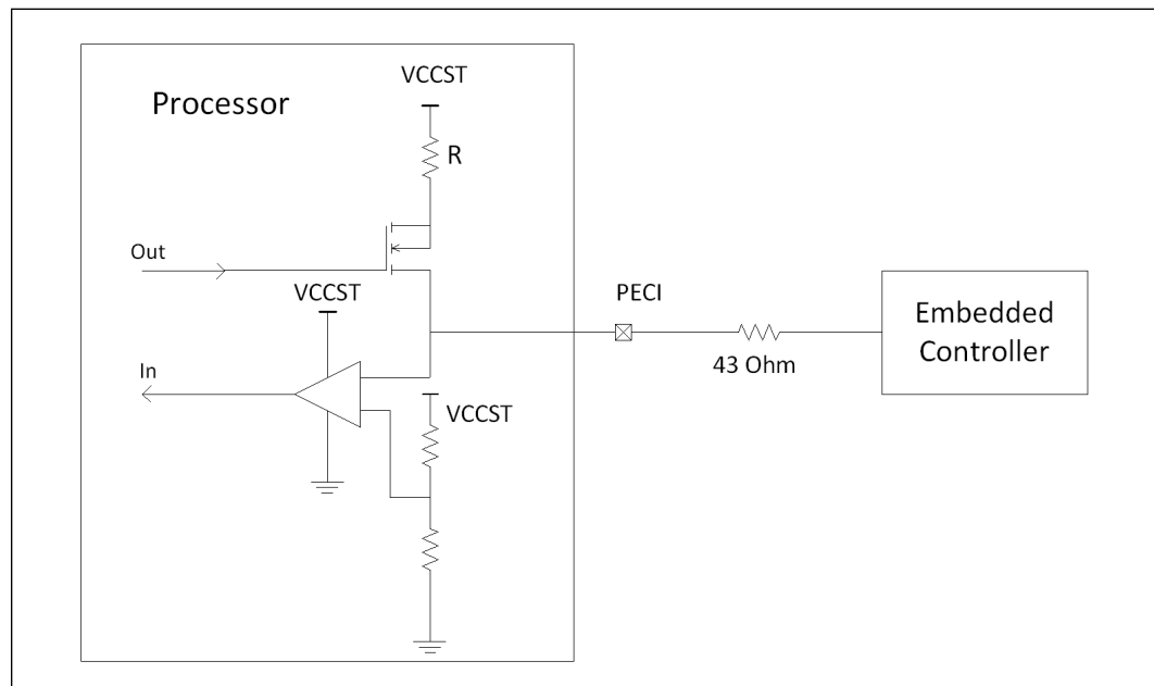
Figure 2-10. Example for PECE EC Connection
