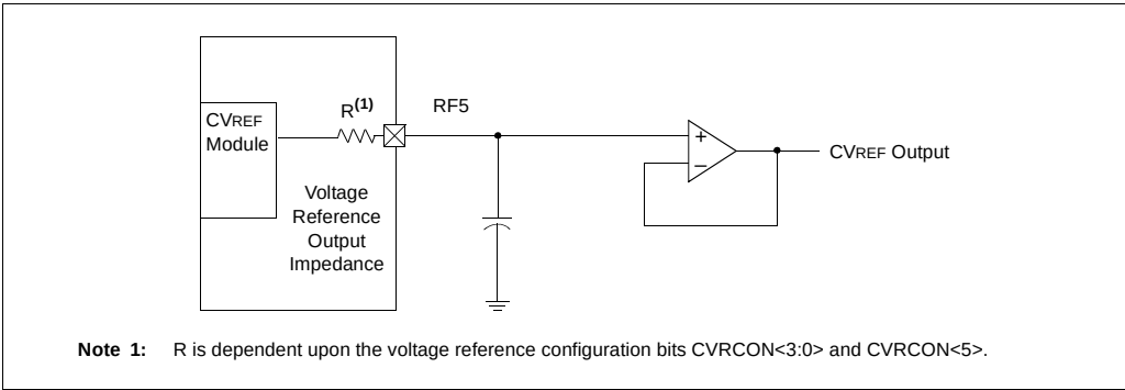
FIGURE 21-2: VOLTAGE REFERENCE OUTPUT BUFFER EXAMPLE
