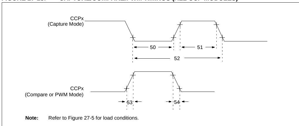
FIGURE 27-13: CAPTURE/COMPARE/PWM TIMINGS (ALL CCP MODULES)
