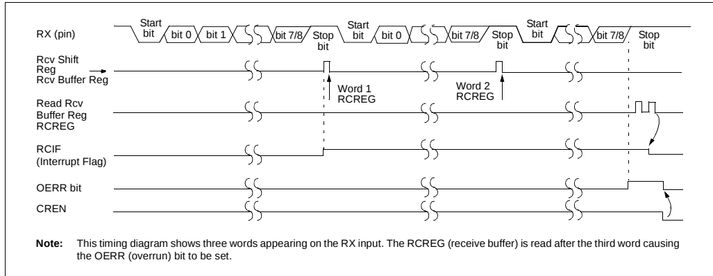
FIGURE 18-6: ASYNCHRONOUS RECEPTION
