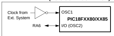
FIGURE 2-5: EXTERNAL CLOCK INPUT OPERATION (ECIO CONFIGURATION)
