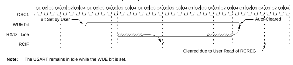
FIGURE 18-7: AUTO-WAKE-UP BIT (WUE) TIMINGS DURING NORMAL OPERATION
