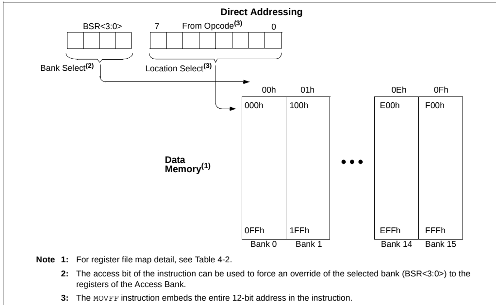
FIGURE 4-8: DIRECT ADDRESSING
