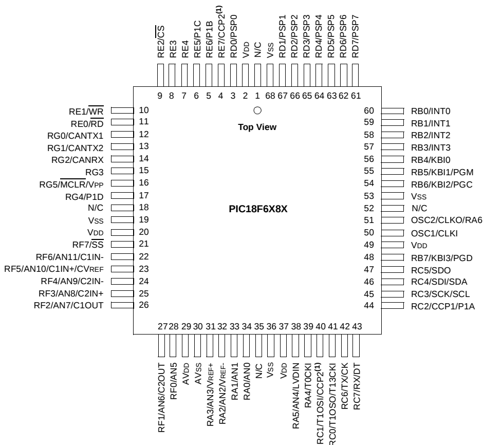
68-Pin PLCC
