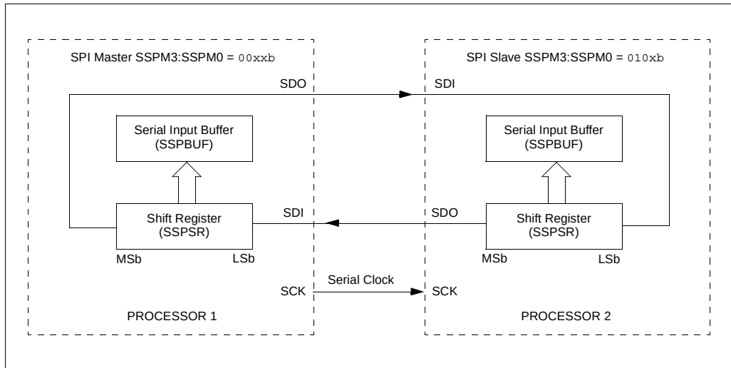
FIGURE 17-2: SPI MASTER/S�AVE CONNECTION
