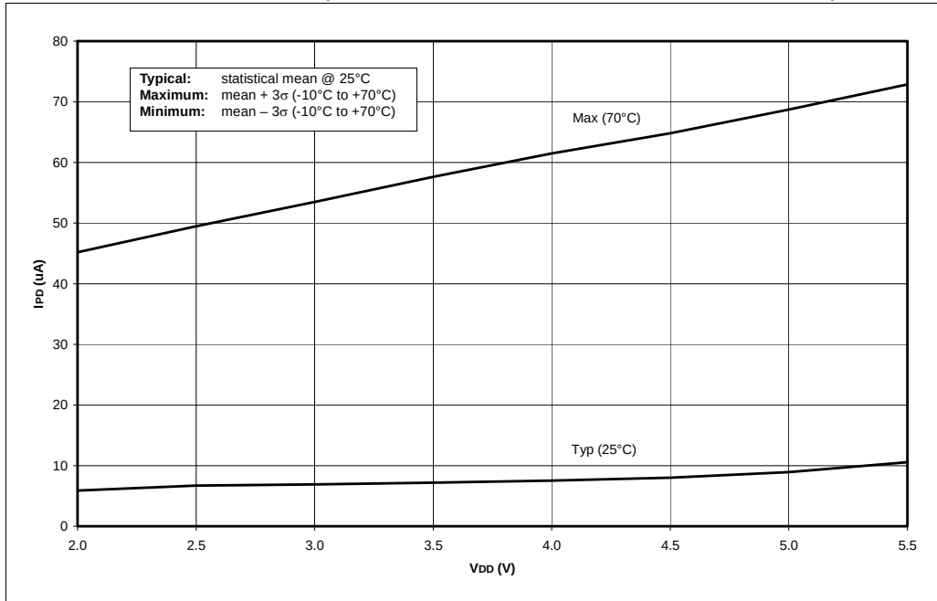
FIGURE 28-17: I_{TOSC} vs. V_{DD} (SLEEP MODE, TIMER1 AND OSCILLATOR ENABLED)
