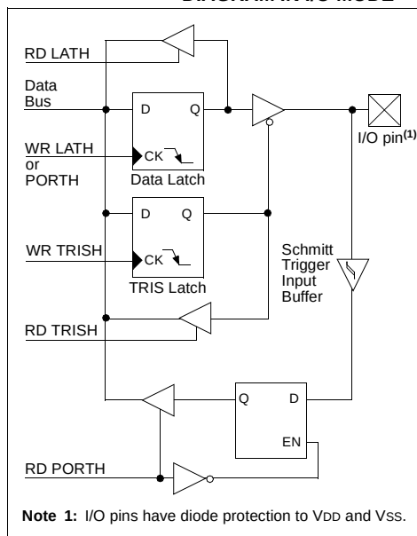
FIGURE 10-22: RH3:RH0 PINS BLOCK DIAGRAM IN I/O MODE
