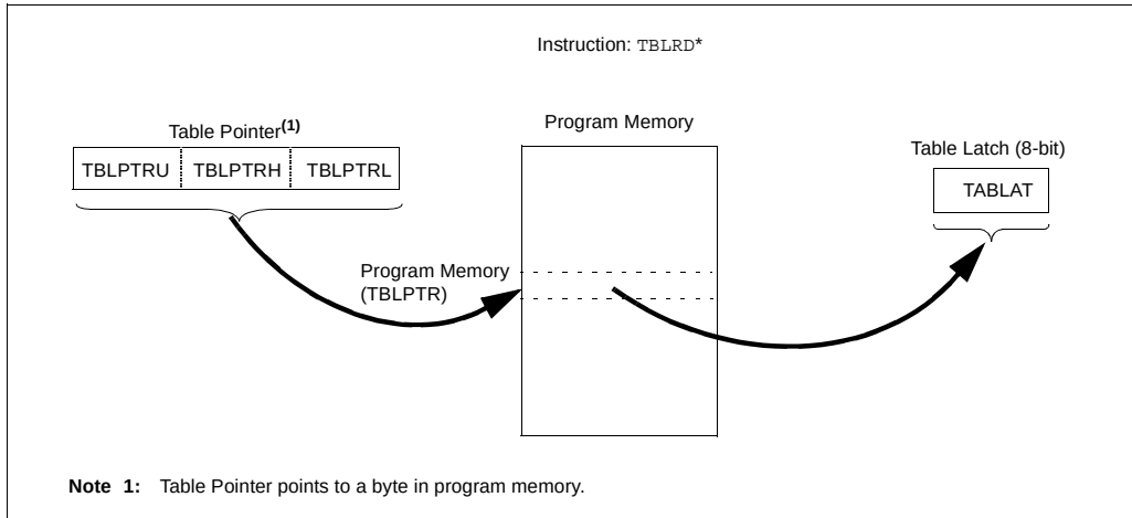
FIGURE 5-1: TABLE READ OPERATION
