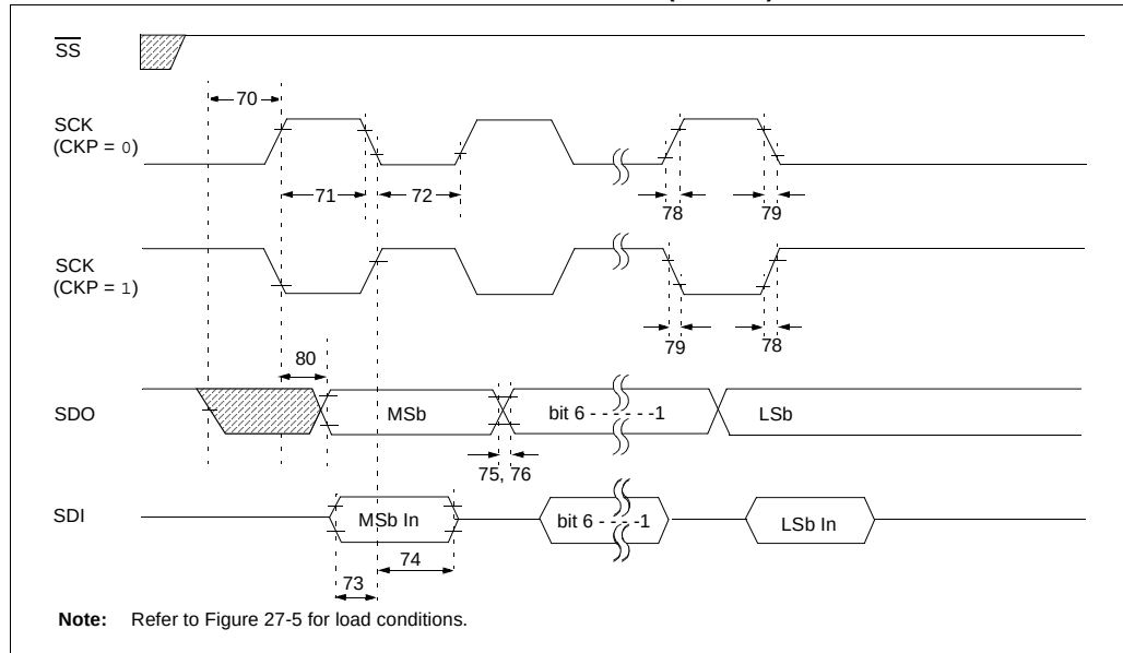
FIGURE 27-15: EXAMPLE SPI MASTER MODE TIMING (CKE = 0)
