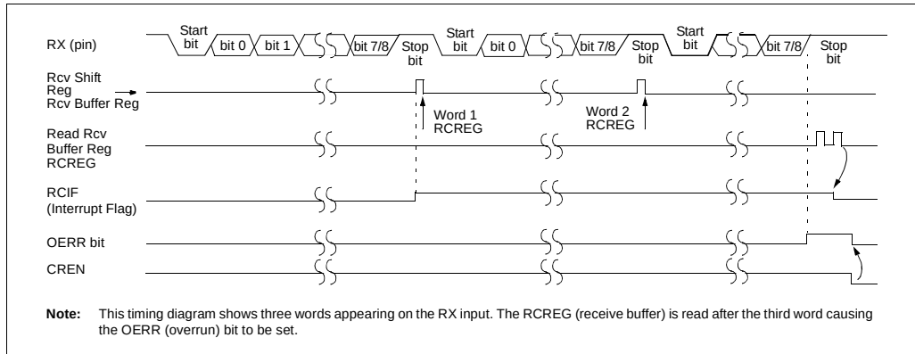
FIGURE 18-6: ASYNCHRONOUS RECEPTION
