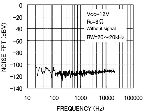
Fig. 12 FFT of Output Noise Voltage
