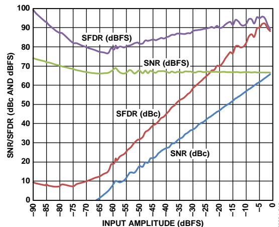
Figure 16. Single Tone SNR/SFDR vs. Input Amplitude ( A_{IN} ), f_{IN} = 70.3 MHz
