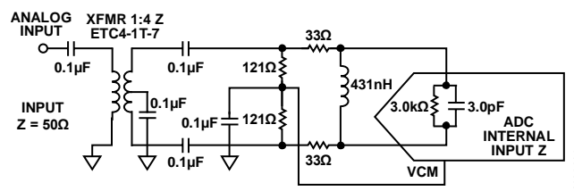
Figure 40. 1:4 Transformer Passive Configuration
