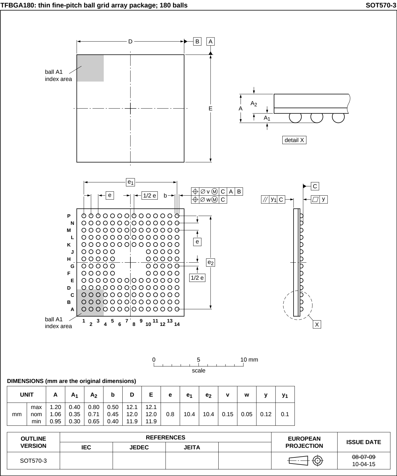
Fig 45. TFBGA180 package
