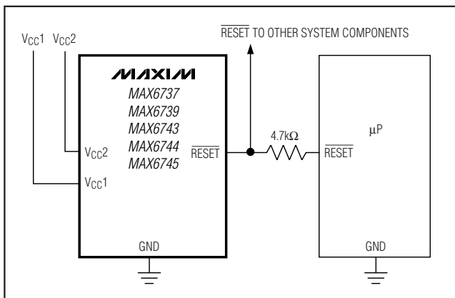
Figure 5. Interfacing to \mu Ps with Bidirectional Reset I/O
