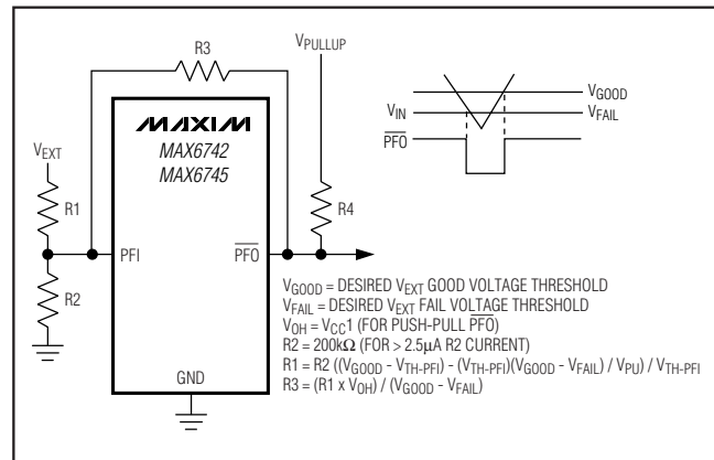
Figure 6. Adding Hysteresis to Power Fail for Push-Pull \overline{PFO}
