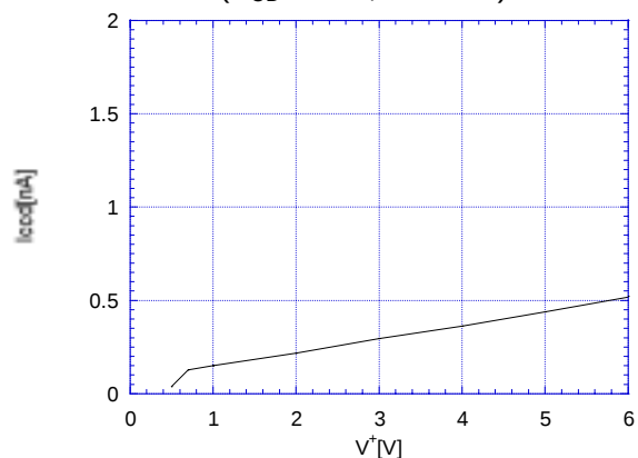
Standby Current vs. Operating Voltage ( V_{CD}=\text{GND} , T_a=25^\circ\text{C} )
