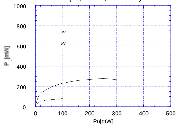
Power Dissipation vs. Output Power ( R_L=32\Omega , T_a=25^\circ\text{C} )
