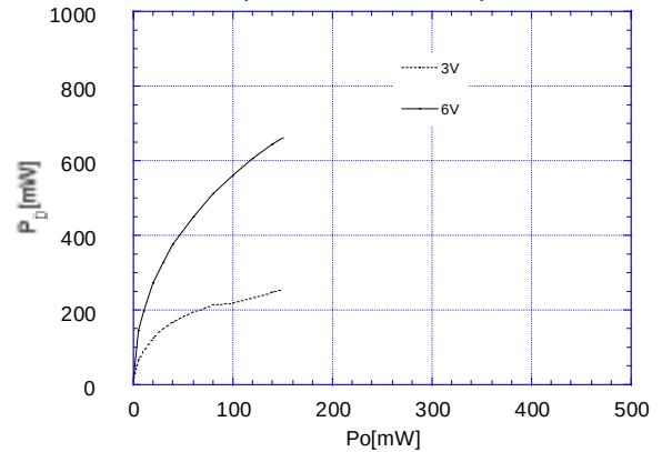
Power Dissipation vs. Output Power ( R_L=8\Omega , T_a=25^\circ\text{C} )
