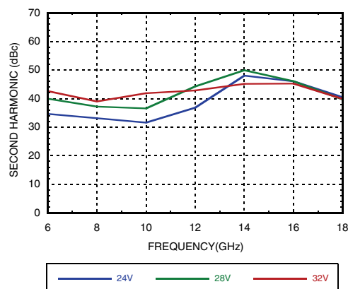
Second Harmonics vs. Supply Voltage
