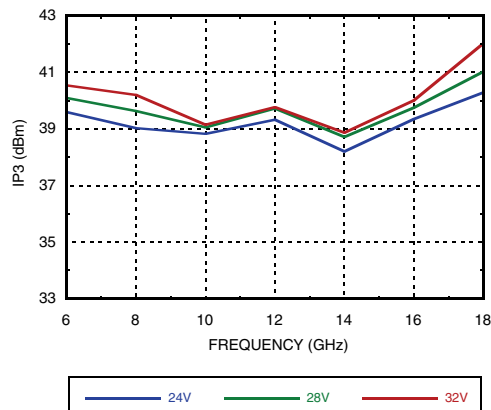
Output IP3 vs. Supply Voltage Pout/tone = +28 dBm
