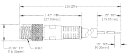
MALE STRAIGHT
