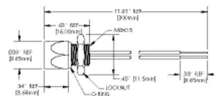
FEMALE RECEPTACLE (ACCOMMODATES THREADED MALE CORDSETS ONLY)
