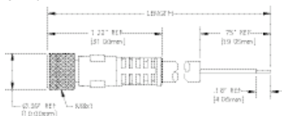
FEMALE STRAIGHT
