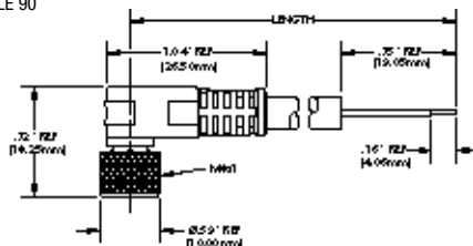
FEMALE 90°
