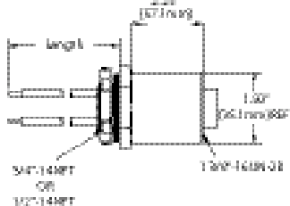
FEMALE RECEPTACLE
