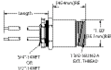
MALE RECEPTACLE
