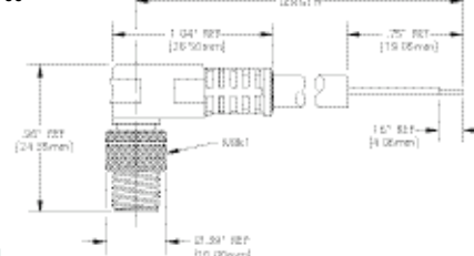
MALE 90°
