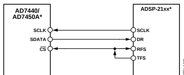
Figure 45. Interfacing to the ADSP-21xx
