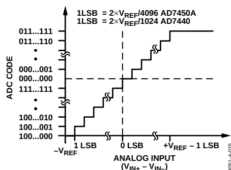
Figure 25. AD7440/AD7450A Ideal Transfer Characteristic
