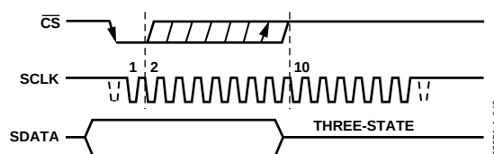
Figure 42. Entering Power-Down Mode
