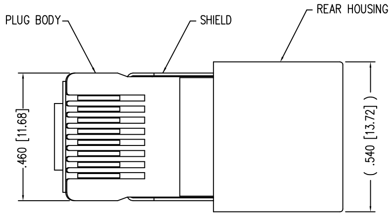
( SHOWN ASSEMBLED )
