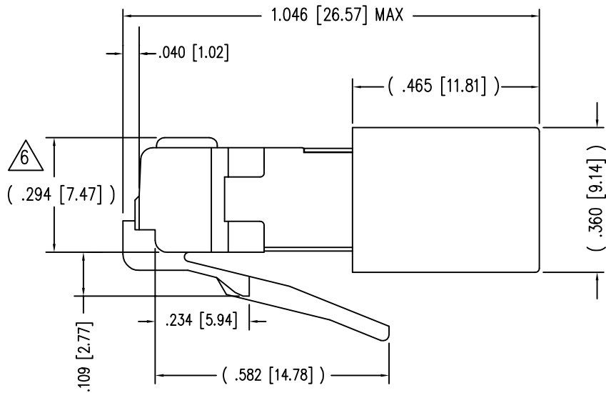
( SHOWN ASSEMBLED )
