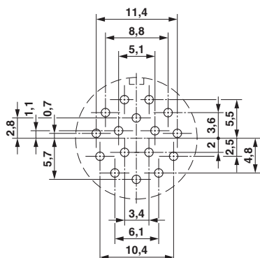
Drilling diagram
