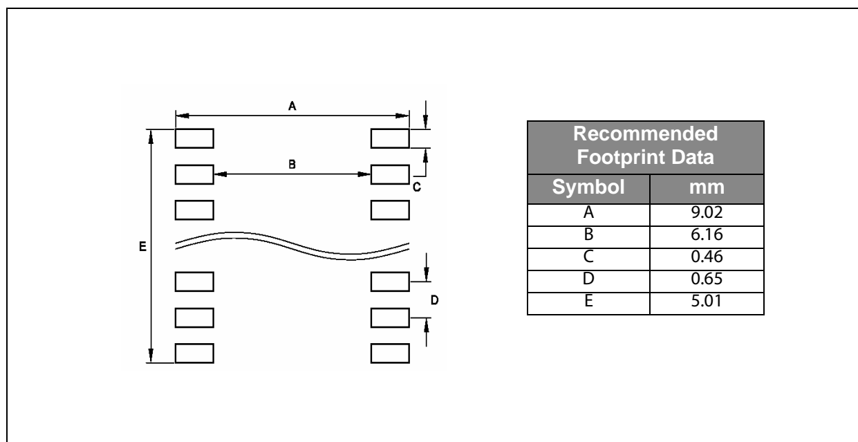
Figure 38: PCB Footprint
