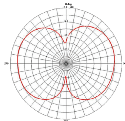
ELEVATION PLANE
