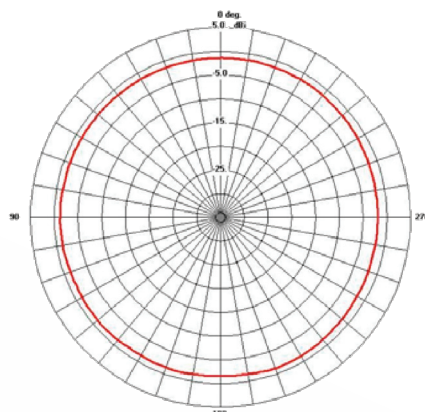
AZIMUTH PLANE
