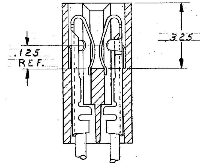
SECTION X-X
