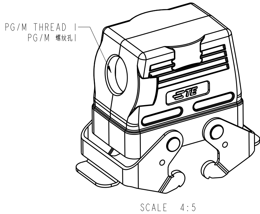
TYPE 1: LOW CONSTRUCTION, SIDE ENTRY WITH STEEL DOUBLE LOCKING 类型1: 低结构, 侧出, 带彩锌双扣
