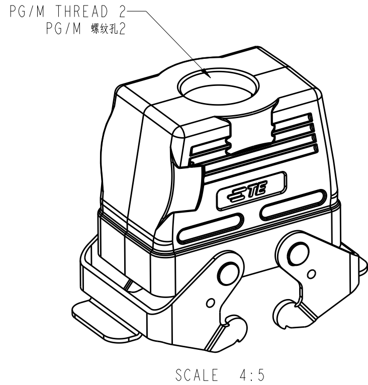
TYPE 2: LOW CONSTRUCTION, TOP ENTRY WITH STEEL DOUBLE LOCKING OTHER SPEC REFER TO TYPE 1 类型2: 低结构, 顶出, 带彩锌双扣, 其它规格参照类型1
