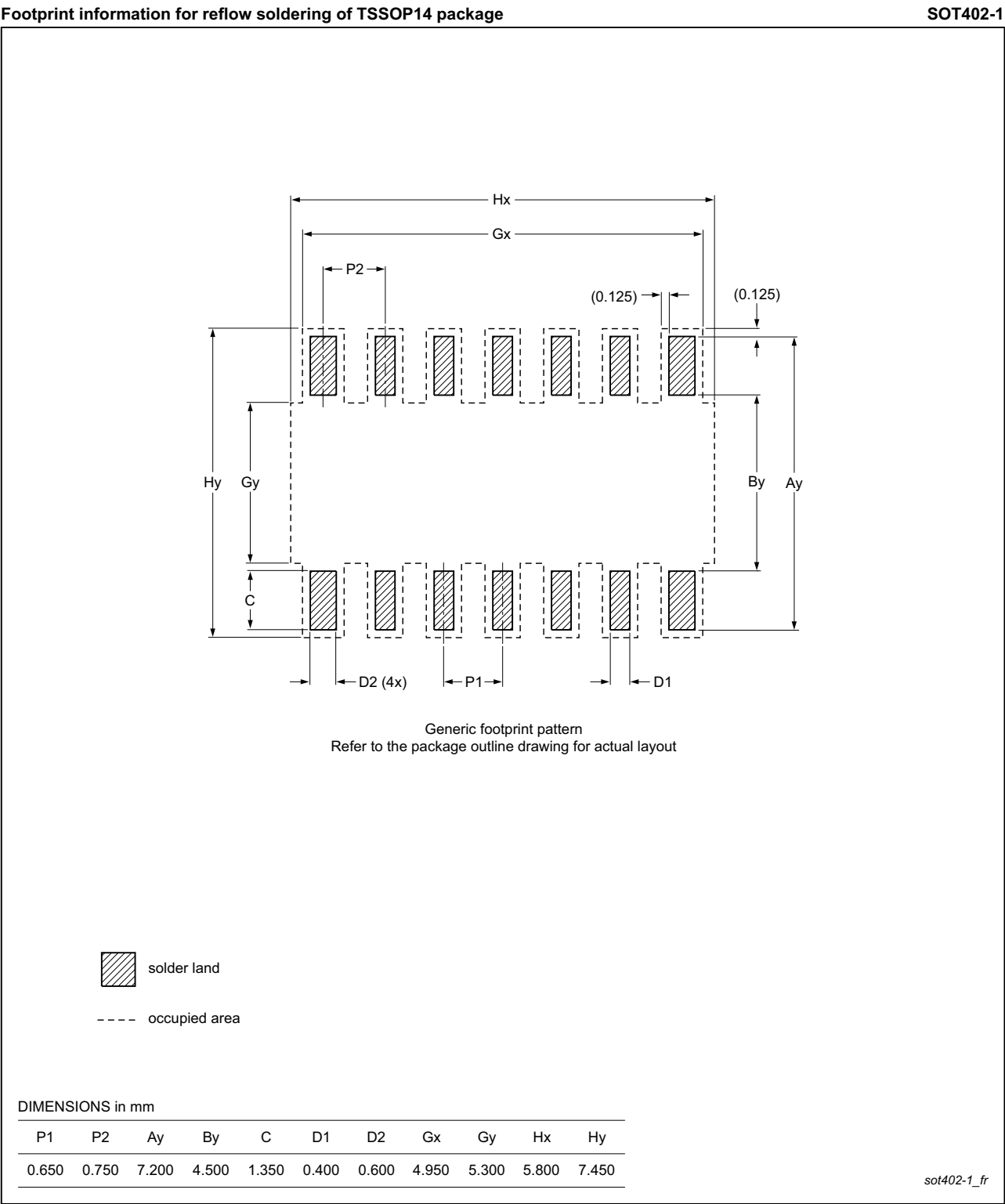
Fig 22. PCB footprint for SOT402-1 (TSSOP14); reflow soldering
