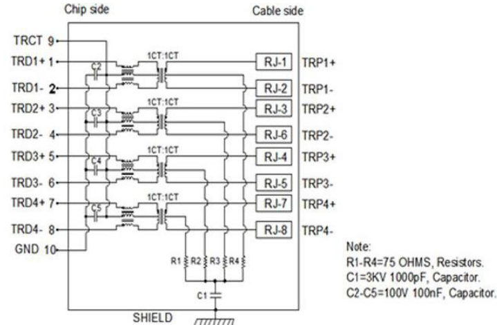
809 (2.5G Base-T)
