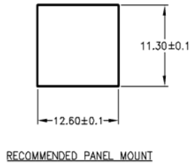
RECOMMENDED PANEL MOUNT
