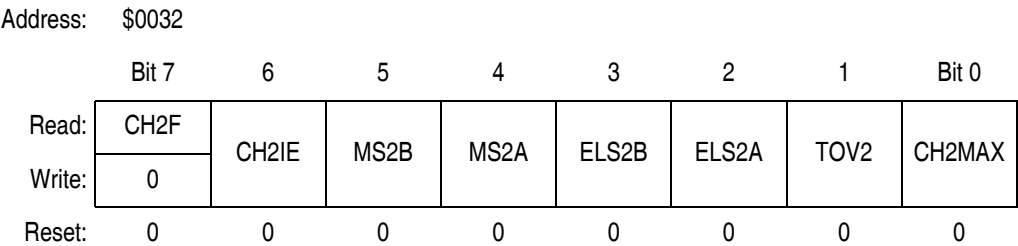
Figure 12-11. TIMB Channel 2 Status and Control Register (TBSC2)
