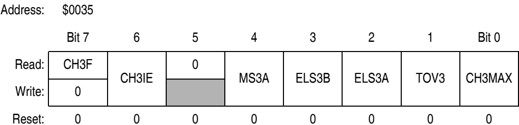
Figure 12-12. TIMB Channel 3 Status and Control Register (TBSC3)
