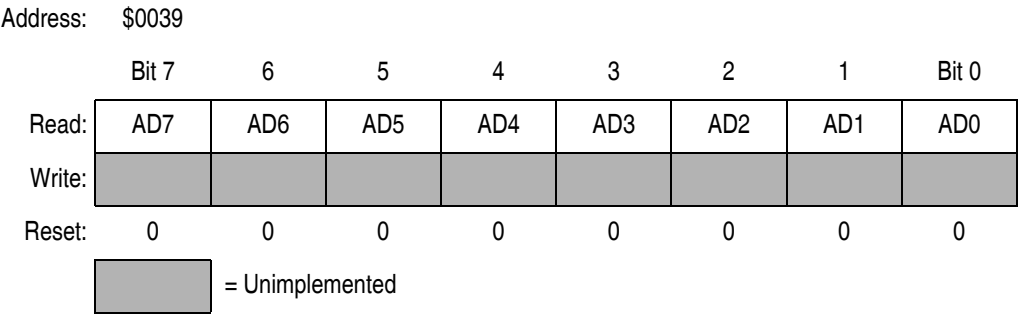
Figure 14-4. ADC Data Register (ADR)
